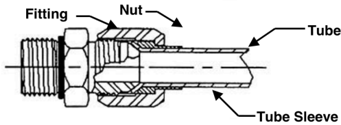
Fig.20 37° Tube Fitting Assembly
